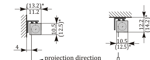
rotary switch
